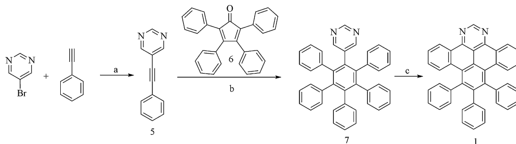
Scheme 2. Reagents and conditions: (a) DIPA, \text{PPh}_3 , \text{PdCl}_2(\text{PPh}_3)_2 , \text{CuI} , DMF, \mu\text{w} , 115 °C, 93%; (b) \text{Ph}_2\text{O} , 260 °C, 44%; (c) \text{FeCl}_3/\text{CH}_3\text{NO}_2 , DCM, 94%.
