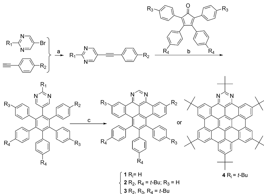
Scheme 1. General route towards pyrimidyl-penta-phenylbenzenes and their cyclodehydrogenation products. (a) Sonogashira coupling, \mu\text{w} ; (b) [2+4] cycloaddition, \text{Ph}_2\text{O} , \mu\text{w} ; (c) cyclodehydrogenation, \text{FeCl}_3 , DCM, \text{CH}_3\text{NO}_2 .
