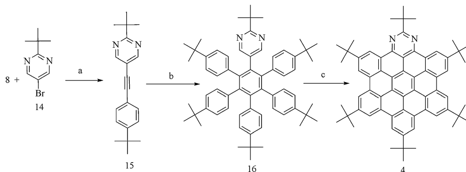
Scheme 5. Reagents and conditions: (a) DIPA, \text{PPh}_3 , \text{PdCl}_2(\text{PPh}_3)_2 , CuI, DMF, \mu\text{w} , 115^\circ\text{C} , 78%; (b) \text{Ph}_2\text{O} , 260^\circ\text{C} , 62%; (c) \text{FeCl}_3/\text{CH}_3\text{NO}_2 , DCM, 60%.
