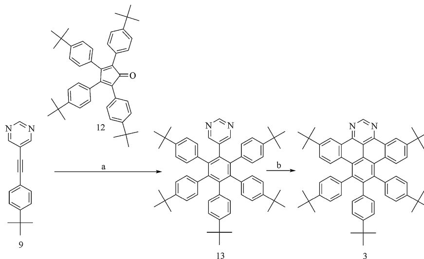
Scheme 4. Reagents and conditions: (a) \text{Ph}_2\text{O} , 260 °C, 46%; (b) \text{FeCl}_3/\text{CH}_3\text{NO}_2 , DCM, 85%.
