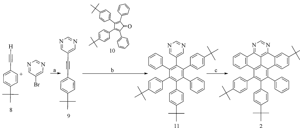
Scheme 3. Reagents and conditions: (a) DIPA, \text{PPh}_3 , \text{PdCl}_2(\text{PPh}_3)_2 , CuI, DMF, \mu\text{w} , 115 °C, 61%; (b) \text{Ph}_2\text{O} , 260 °C, 52%; (c) \text{FeCl}_3/\text{CH}_3\text{NO}_2 , DCM, 90%.
