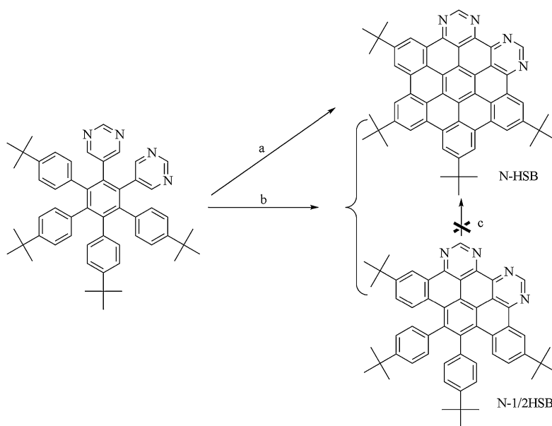
Scheme 6. Reagents and conditions from Refs. 25 and 26 . (a) \text{AlCl}_3 , \text{CuCl}_2 , \text{CS}_2 , rt, 49%; (b) \text{FeCl}_3/\text{CH}_3\text{NO}_2 , DCM, rt; N-HSB (35%)+N-1/2HSB (32%); (c) \text{AlCl}_3/\text{CuCl}_2 or \text{FeCl}_3 .
